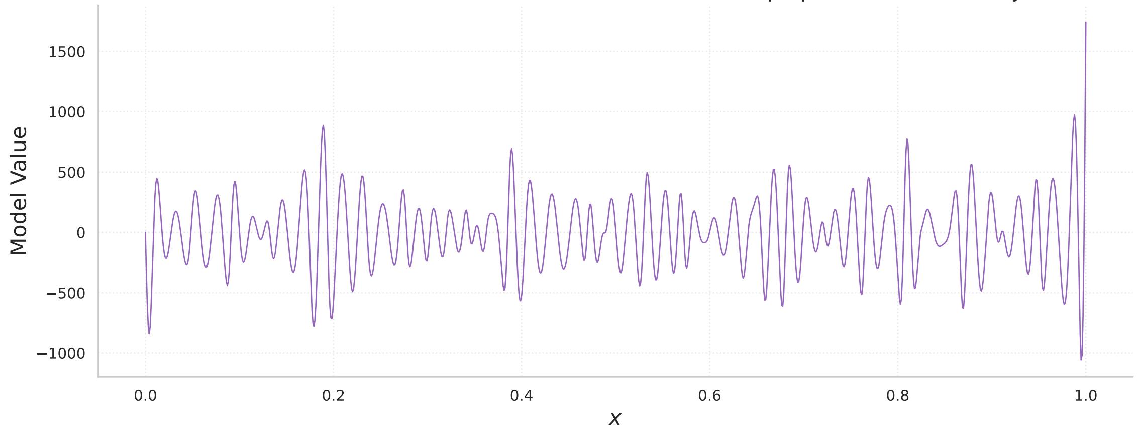
The Confidence-Set Model (data fit relaxed to a 95% CI, properties still hit exactly)
