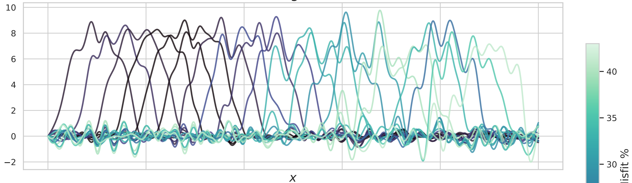
Resolving Kernels
