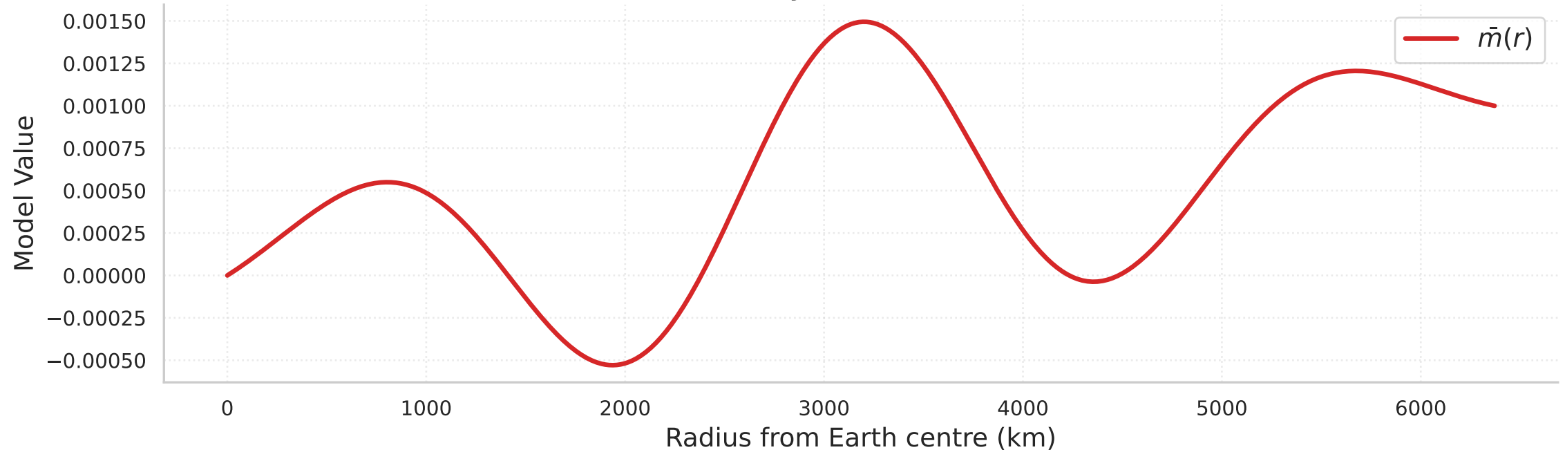
True Synthetic Model
