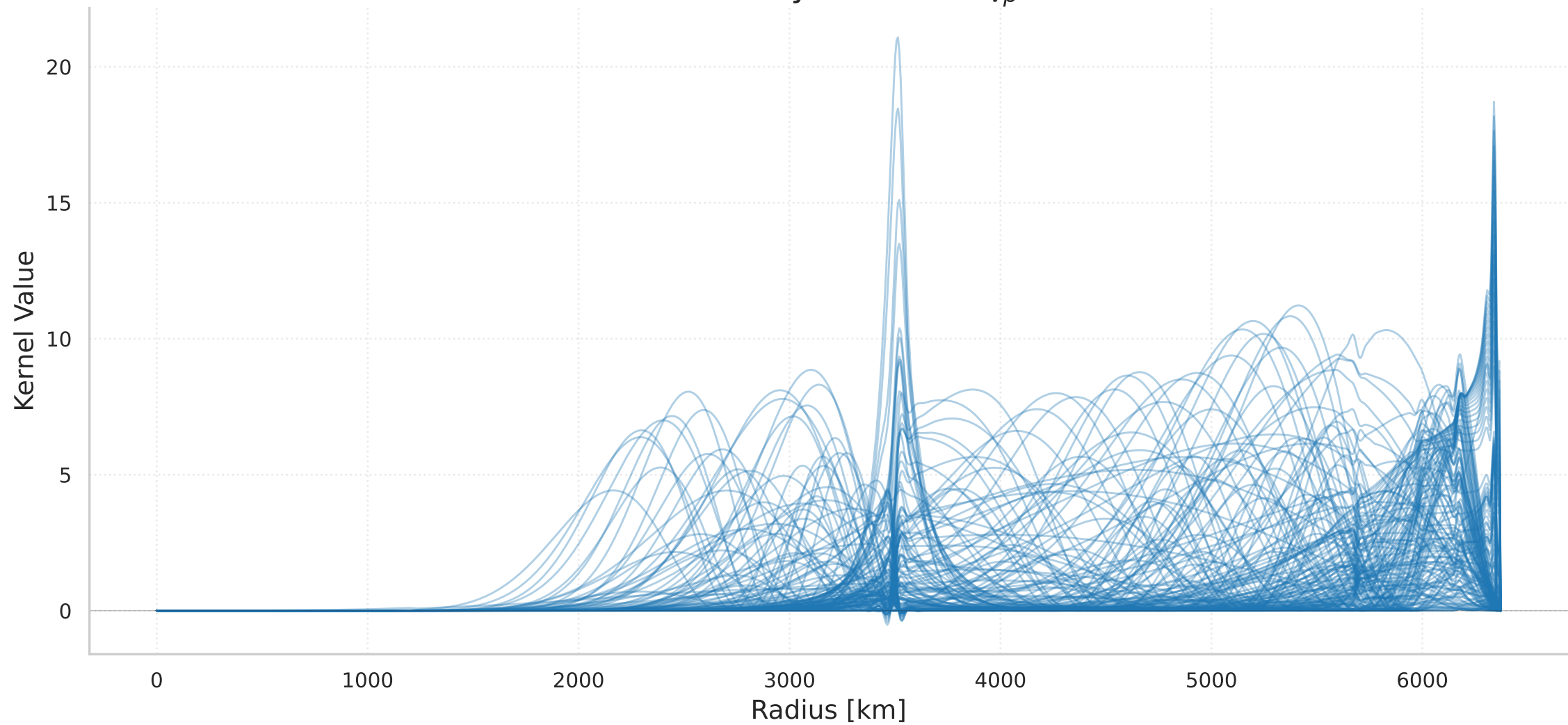
Sensitivity Kernels: K_{vp}
