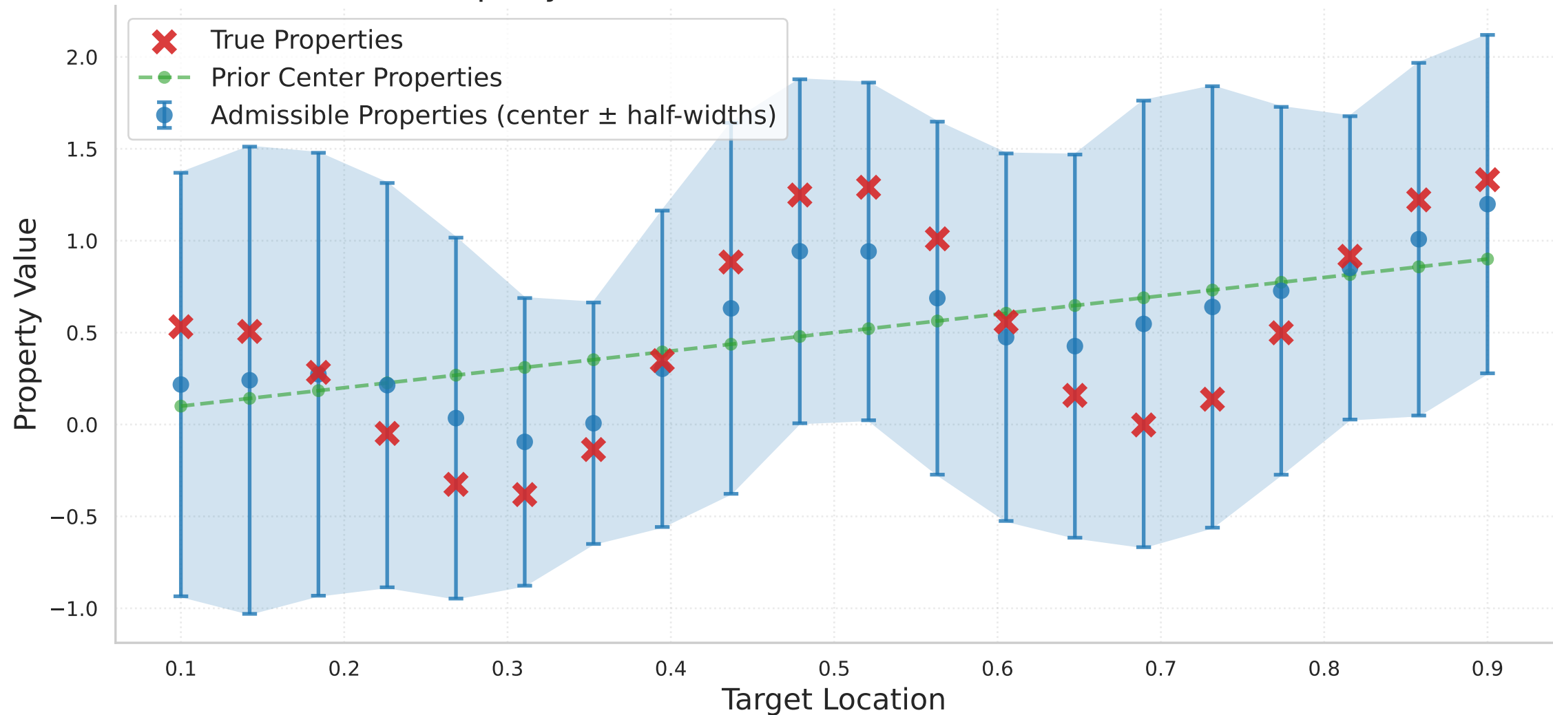
Property Inference Results (DLI — Basis-Free KKT)
