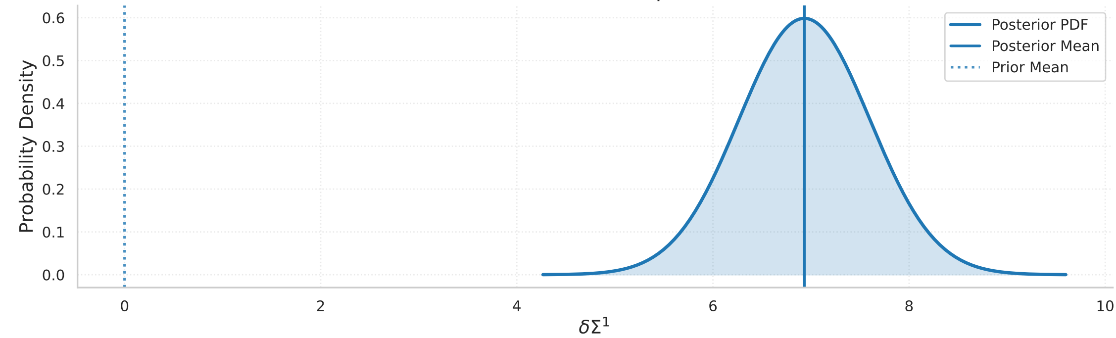
Model Posterior: \delta \Sigma^1 component (CMB)
