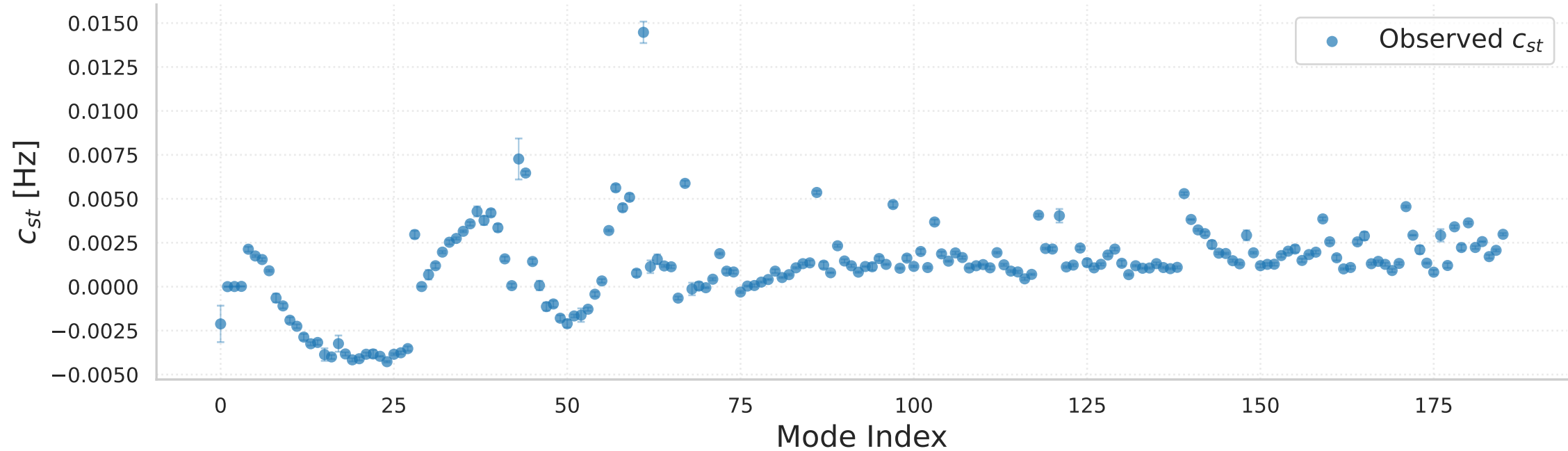
Observed Splitting Coefficients: s = 2, t = 0 (186 modes)
