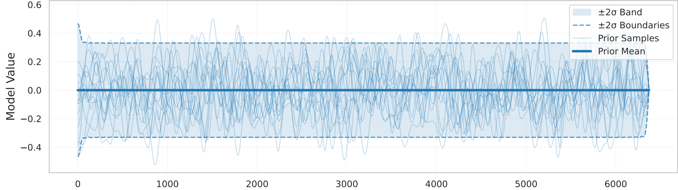
Prior Measure: \delta v_\rho component
