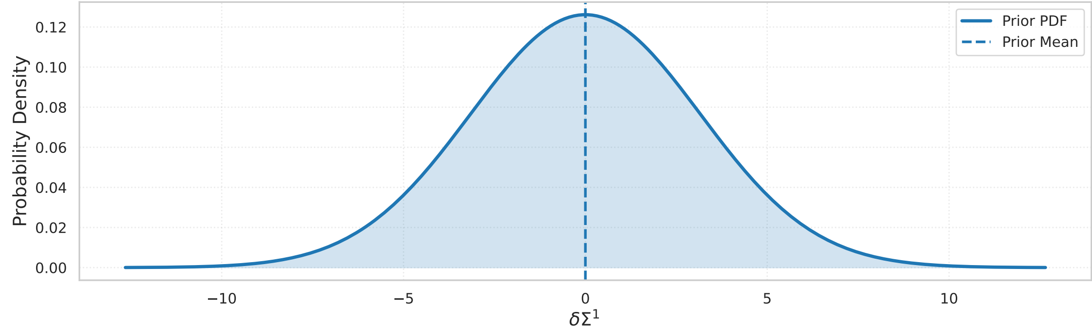
Prior Measure: \delta \Sigma^1 component (CMB)
