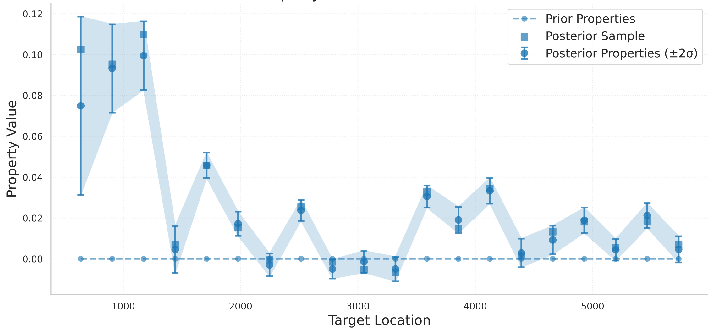
Property Inference Results (RTO)
