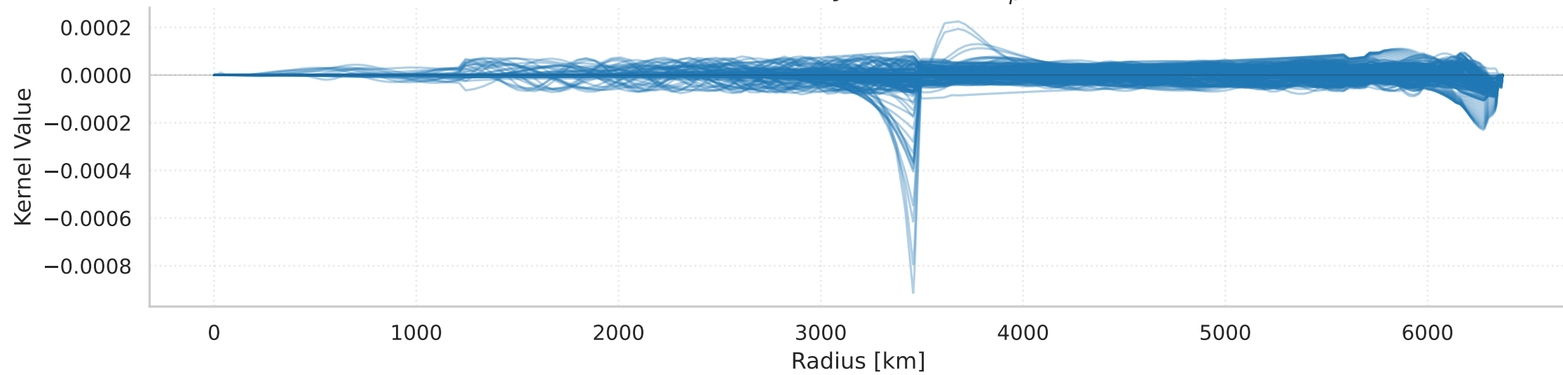
Sensitivity Kernels: K_{\Sigma^0} (ICB)
