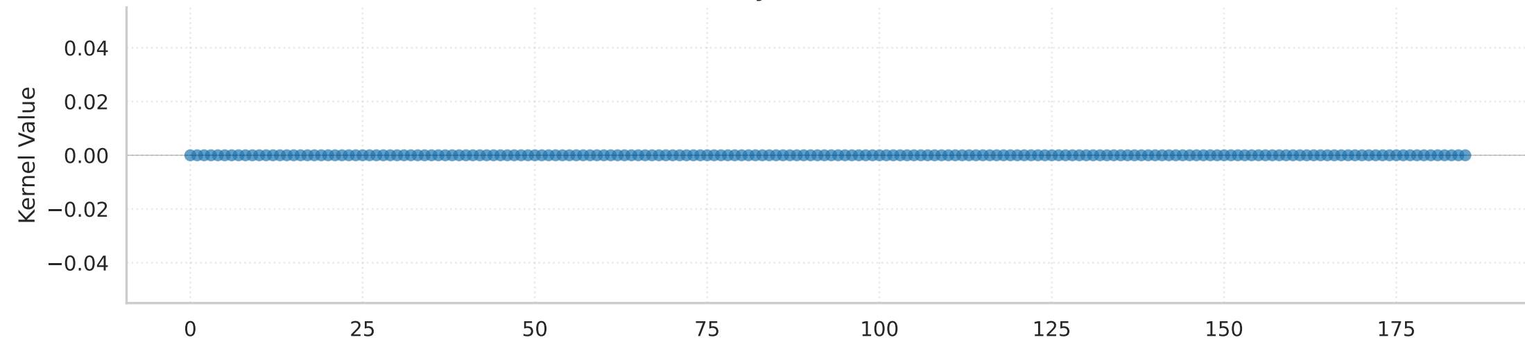
Sensitivity Kernels: K_{\Sigma^0} (ICB)
