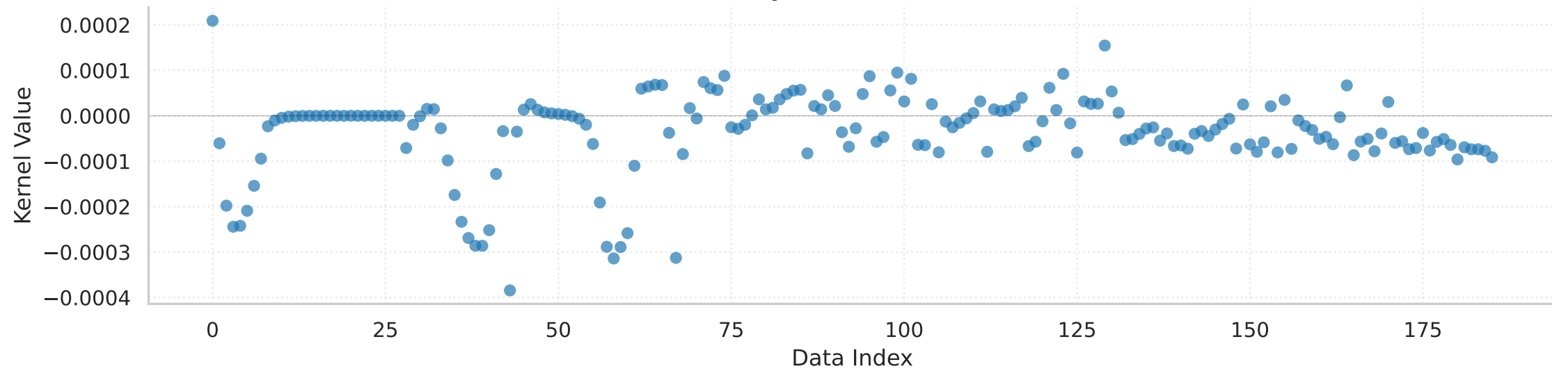
Sensitivity Kernels: K_{\Sigma^1} (CMB)
