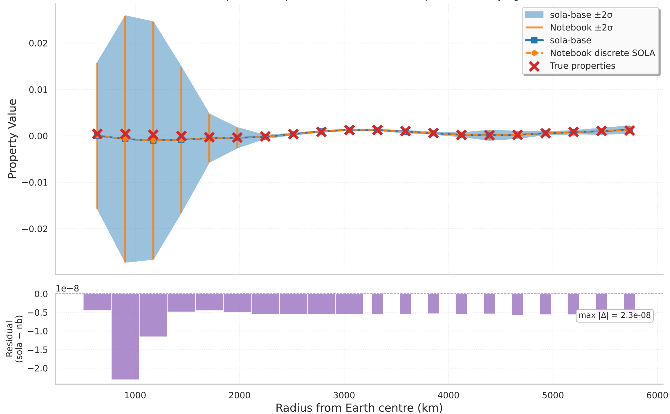
sola-base and Notebook Discrete SOLA — Earth Property Estimates (two independent implementations; lines overlap because they agree)
