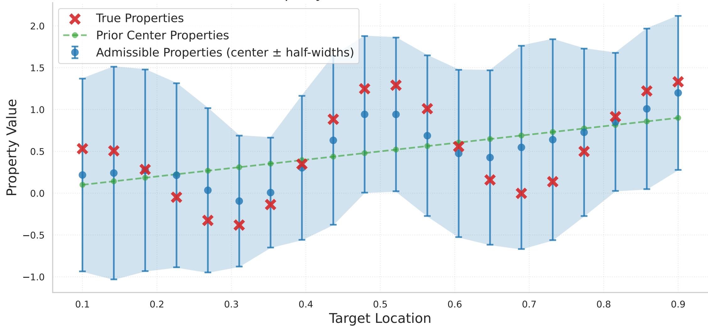
Property Inference Results (DLI)
