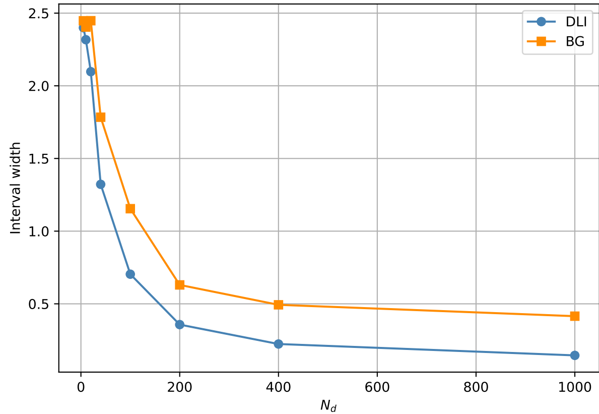
Admissible Interval Widths vs N_d
