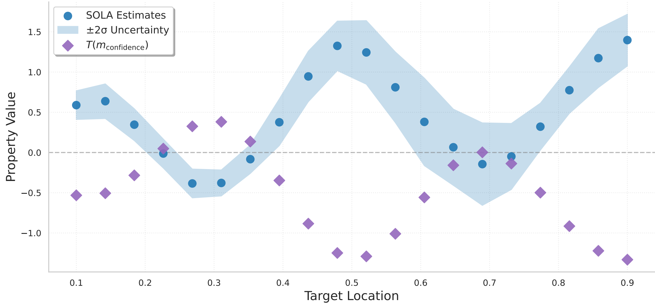
Confidence-Set Model: Achieved Properties vs. SOLA
