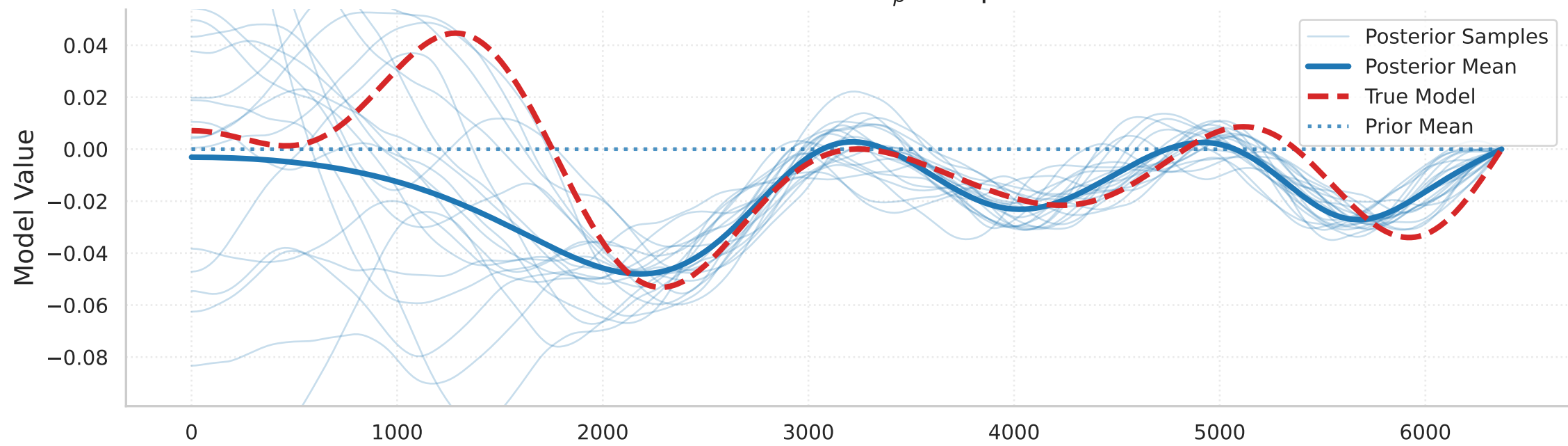
Model Posterior: \delta v_p component
