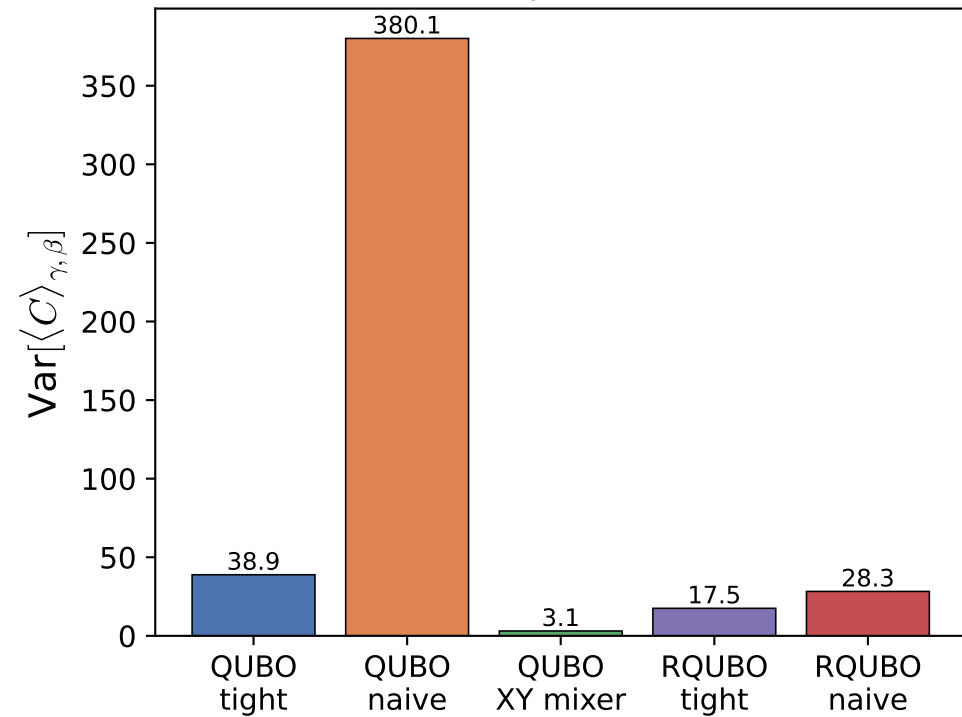
Landscape variance
