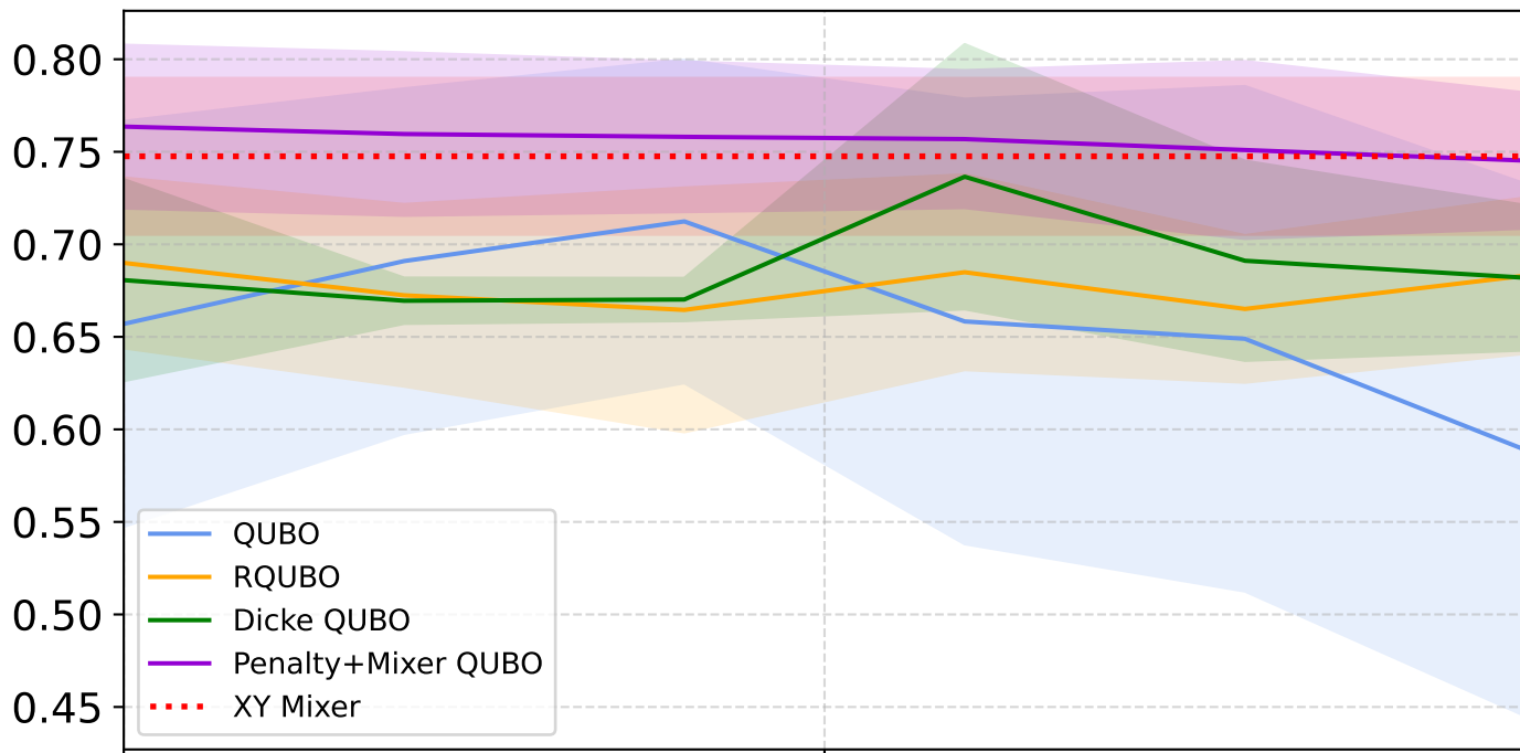
Approximation Ratio
