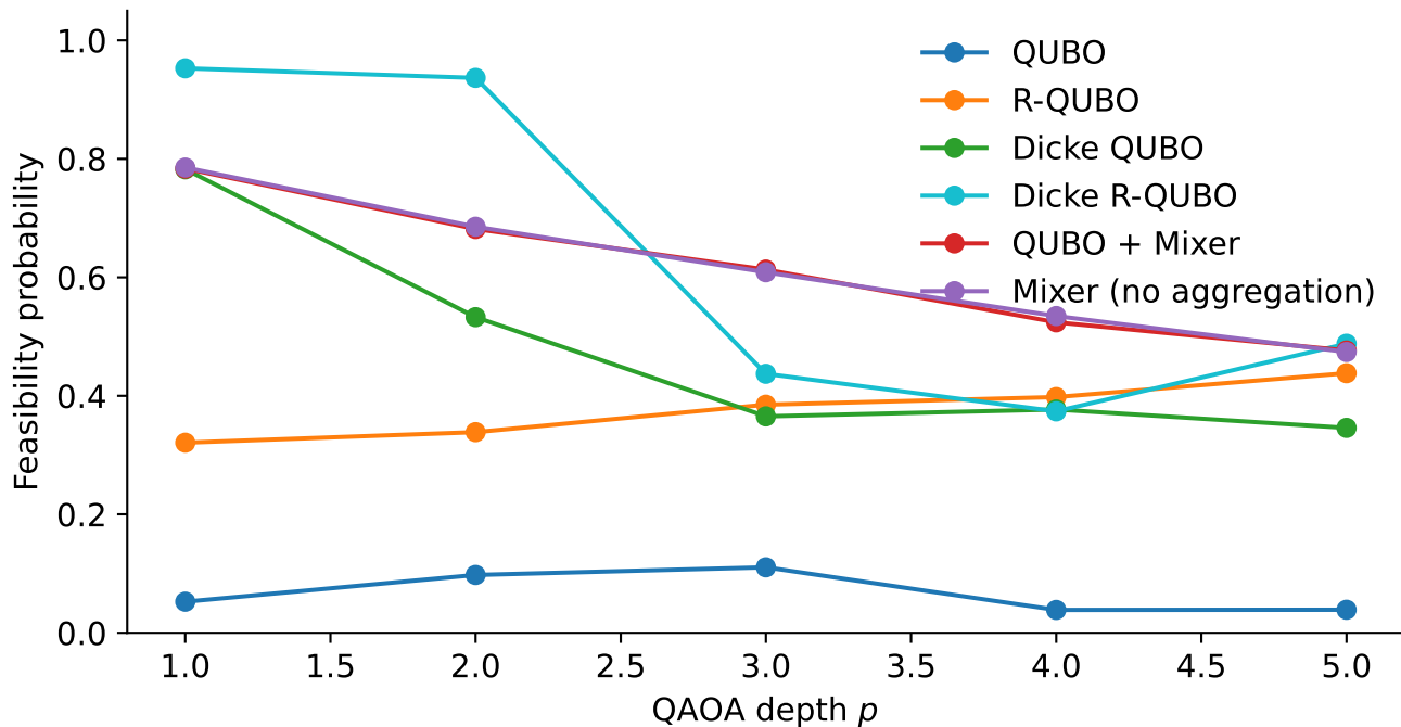
Feasibility vs p (ibm_boston noise)
