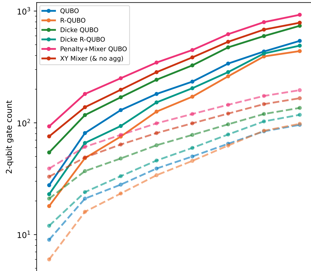
vs graph size
