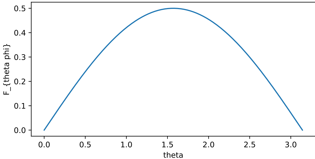
Berry curvature density on CP^1
