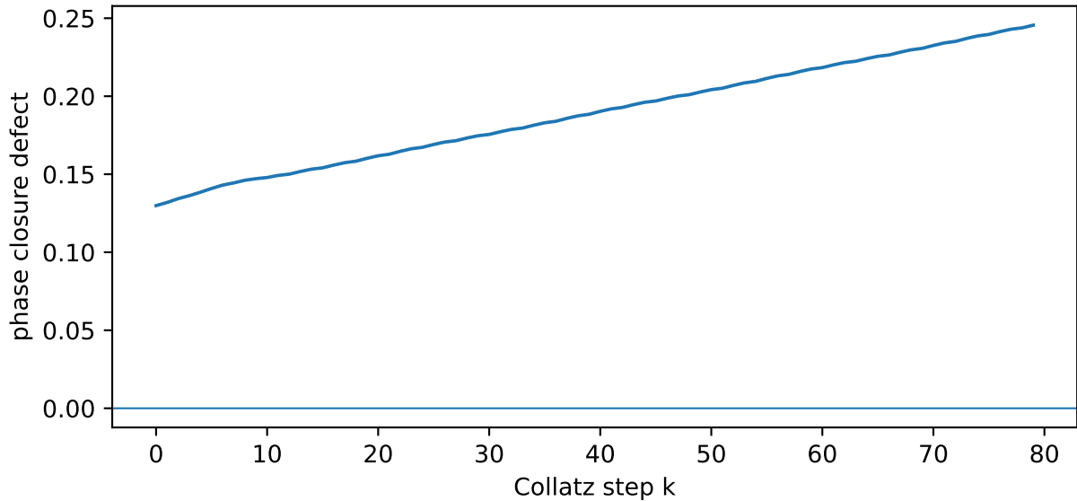
Euler-Berry-Lambda-neutrino closure defect
