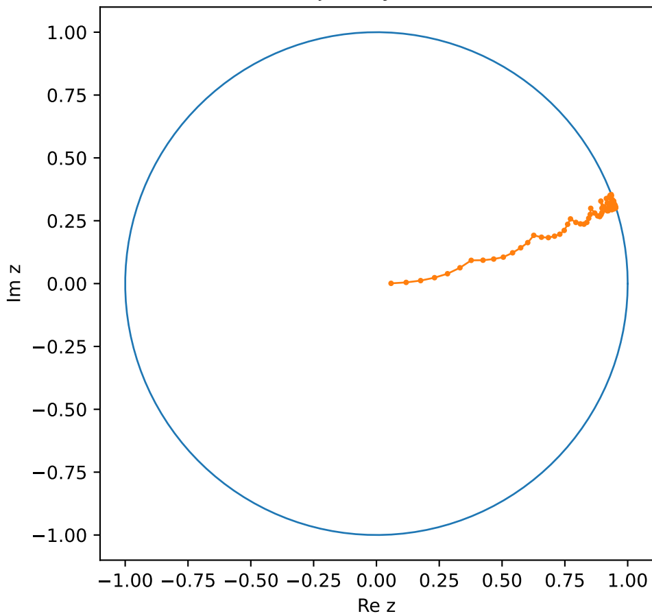
Collatz-driven trajectory on the Poincare disk
