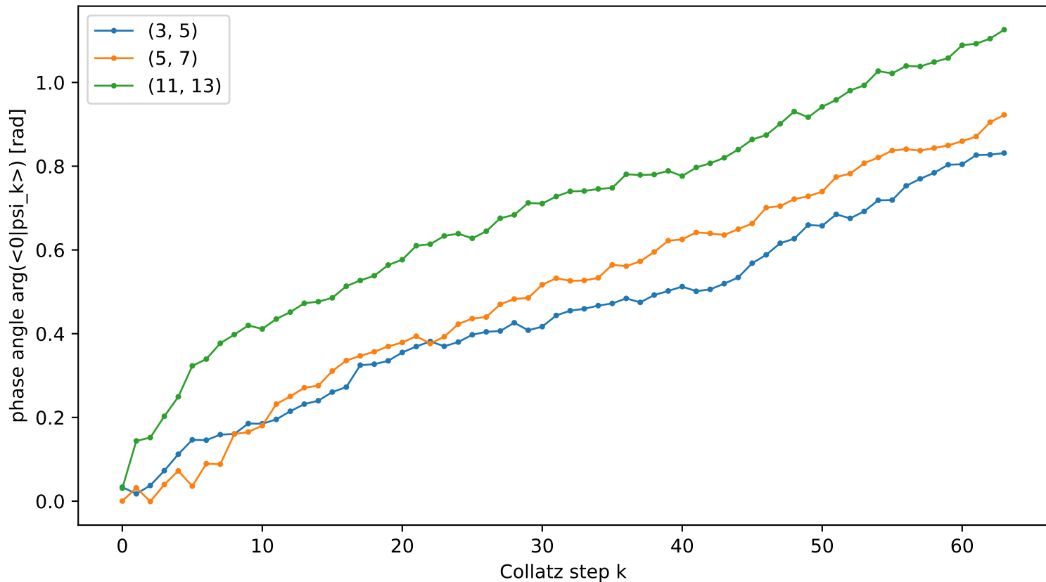
Intention-phase Floquet trace for twin-prime seeds
