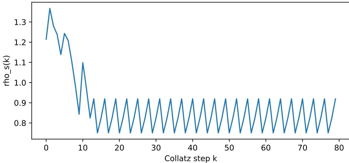
Twin-prime Collatz rhythm
