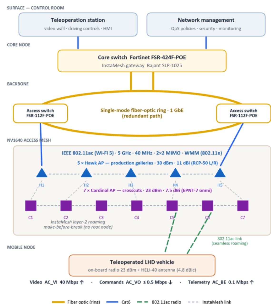
Figure 1. Network architecture: control room, fiber-optic ring and 802.11ac access mesh.
