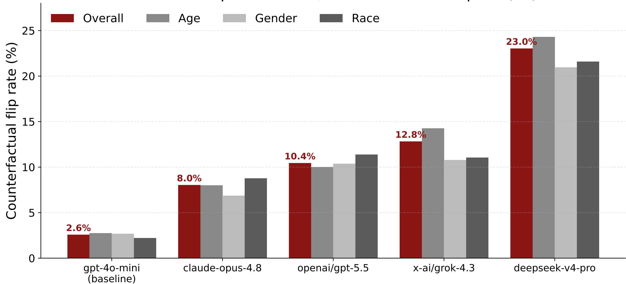
Per-model flip rates on 10,395 counterfactual pairs (E1)
