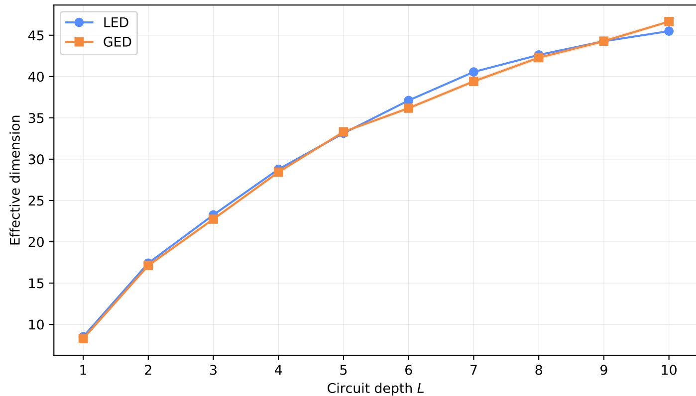
Un-normalized effective dimension
