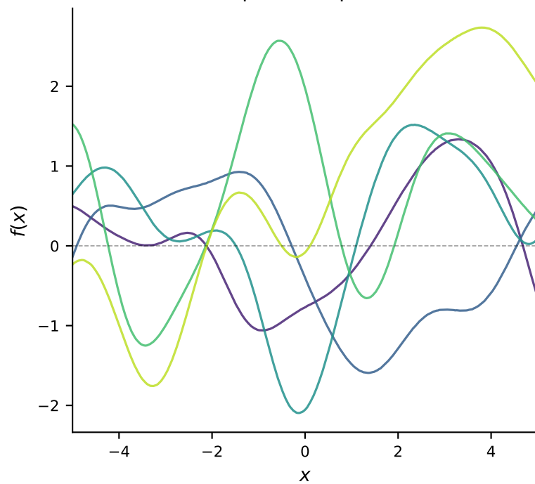
RBF (Squared Exponential)
