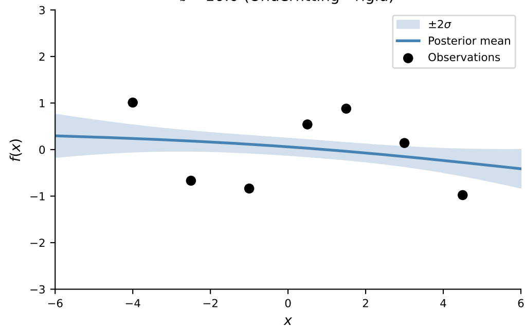
\ell = 10.0 (Underfitting - rigid)
