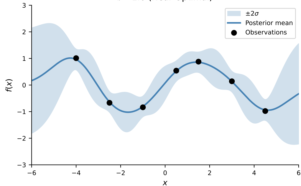
\ell = 1.0 (Near Optimal)
