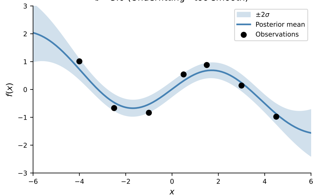
\ell = 3.0 (Underfitting - too smooth)
