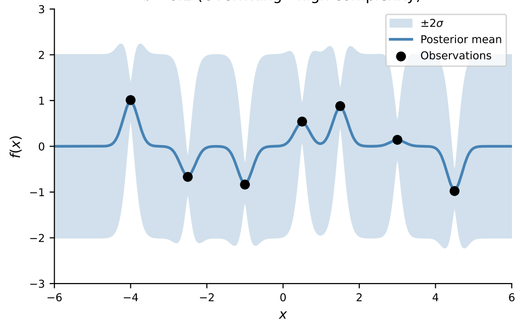
\ell = 0.2 (Overfitting - high complexity)
