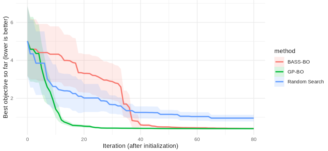
Mean Convergence Across 25 Seeds (d=2)
