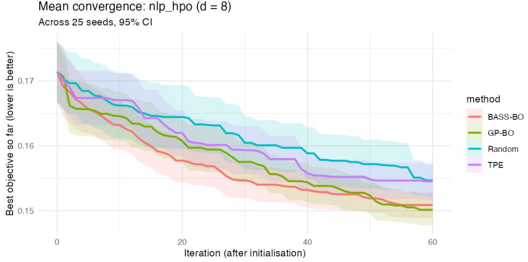
Figure 6.12: The real task: mean best-so-far validation error per iteration across 25 seeds, budget 60 evaluations after a shared initial design of 17 points; shaded bands are 95% confidence intervals across seeds.
