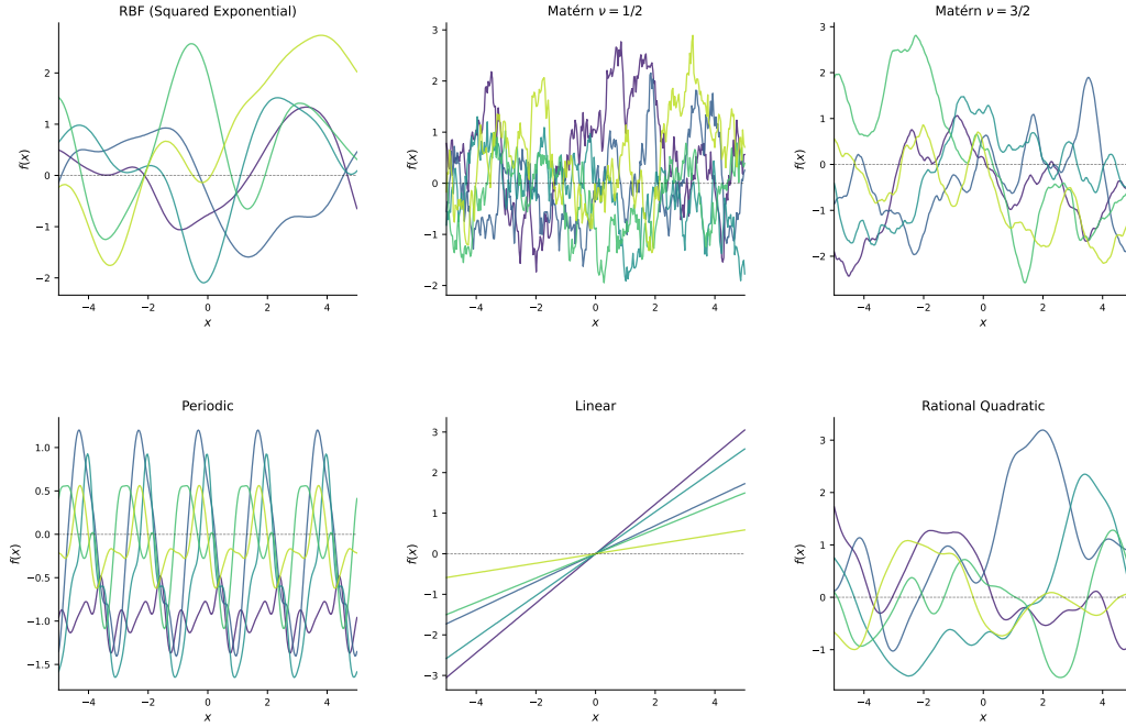
Figure 1.2: Sample paths from a zero-mean Gaussian process under six kernel functions: the RBF (squared exponential), Matérn \nu = 1/2 , Matérn \nu = 3/2 , periodic, linear, and rational quadratic kernels. Each colored trajectory represents an independent sample from the process.
