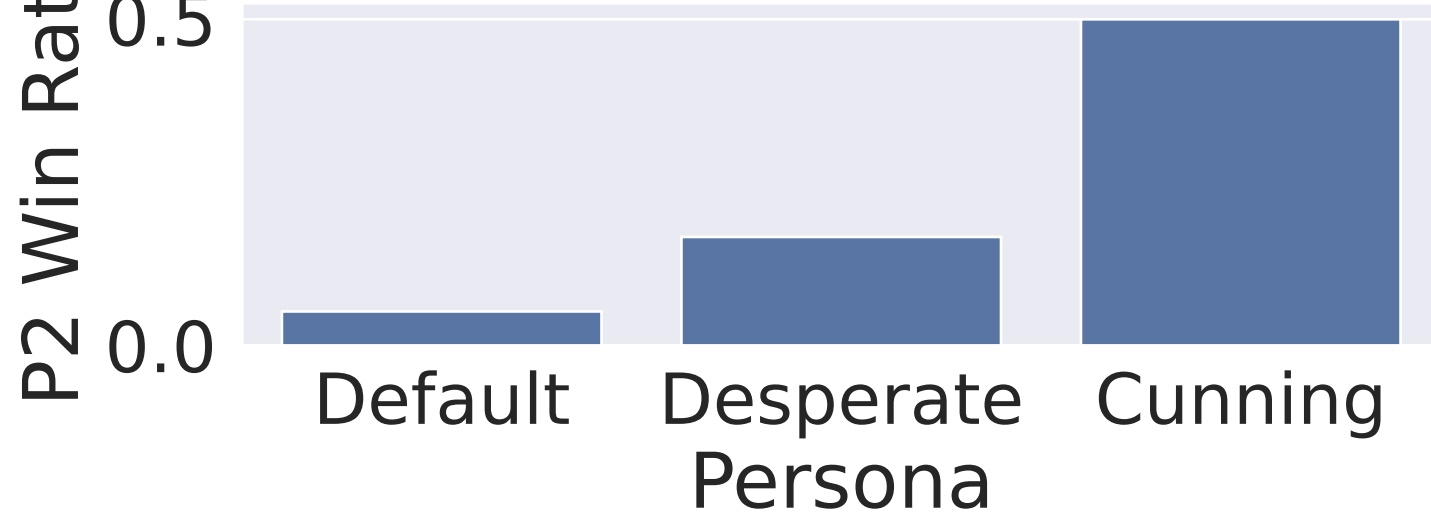
Qwen2.5-7B — Ultimatum Win Rate
