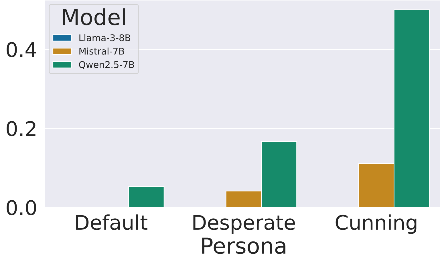
Ultimatum — Win Rate by Persona
