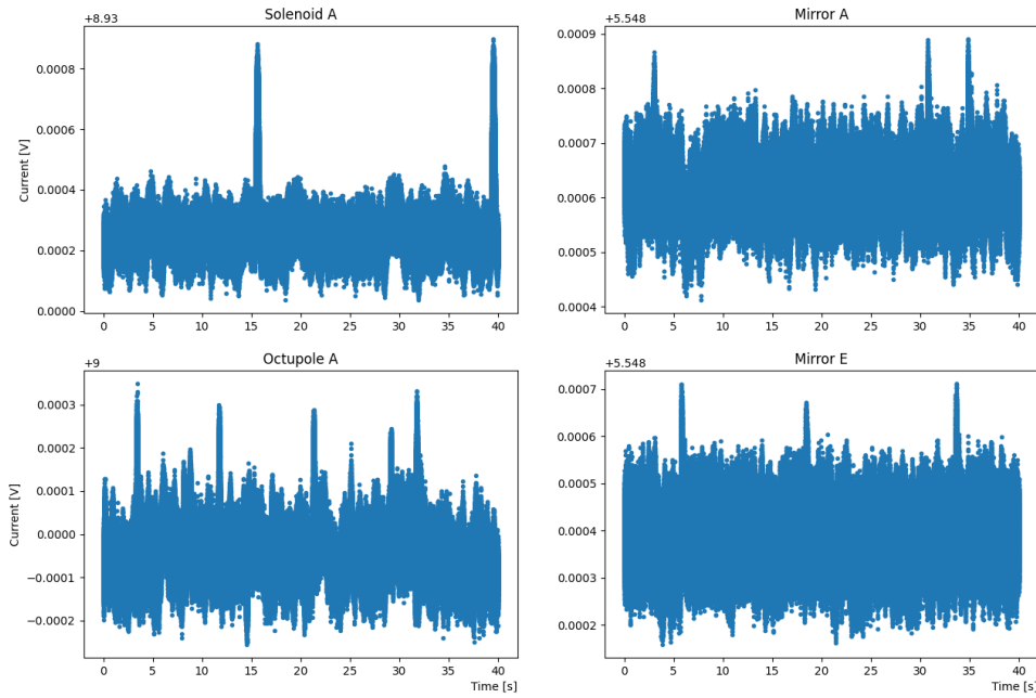
Figure 4.13: Example of DCCTs traces for a total of 40 second of acquisition. The units on the y-axis are Volts, since the DCCT provides a \pm 10 V output. The traces have been converted into Ampere units and the amplitude of the glitches has been used to study possible discrepancies on the measurement induced by changes in the magnetic field minimum
