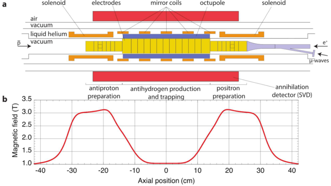
Figure 2.4: Scheme of the ALPHA2 Penning-Malmberg trap (top) and on-axis magnetic field profile for axial confinement of the antihydrogen atoms (bottom).
