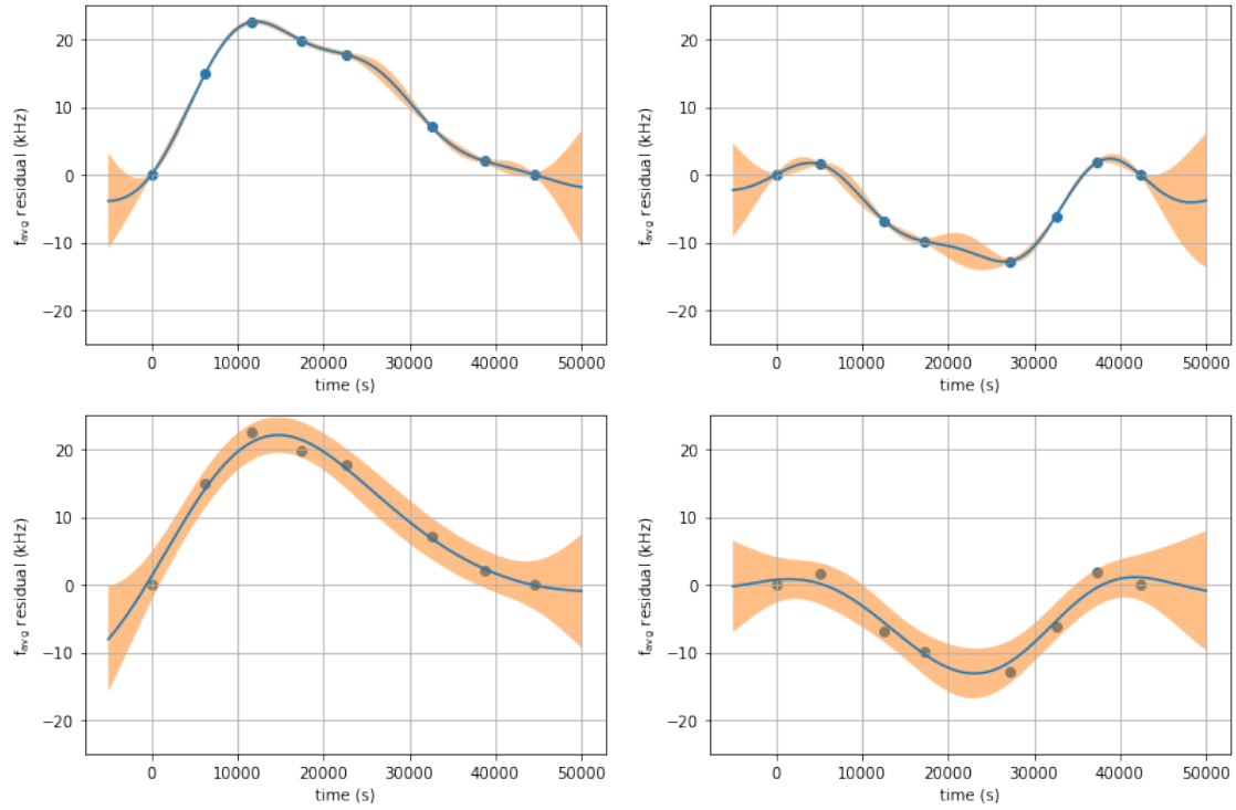
Figure 4.12: Interpolation of the cb frequency markers (points) with Gaussian Process Regression for Series 7 (left) and Series 8 (right). The linear trend is removed before interpolation (detrending is such that the ordinates of the first and last points are zero). The abscissa is the time of the repetition in seconds and the ordinate is the residual w.r.t. the linear trend of the frequency markers, in kHz. The band represents the 95% confidence interval. Top and bottom figures are obtained with different settings for the input noise, without significant changes in the estimate of the systematic uncertainty. The top plots correspond to the settings used for the estimate in Tab. 5.2
