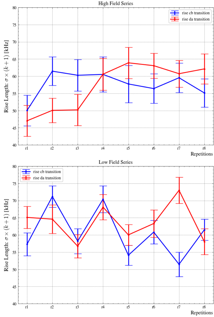
Figure 4.14: Length of the rising edge when letting it vary repetition by repetition (not the nominal configuration).
