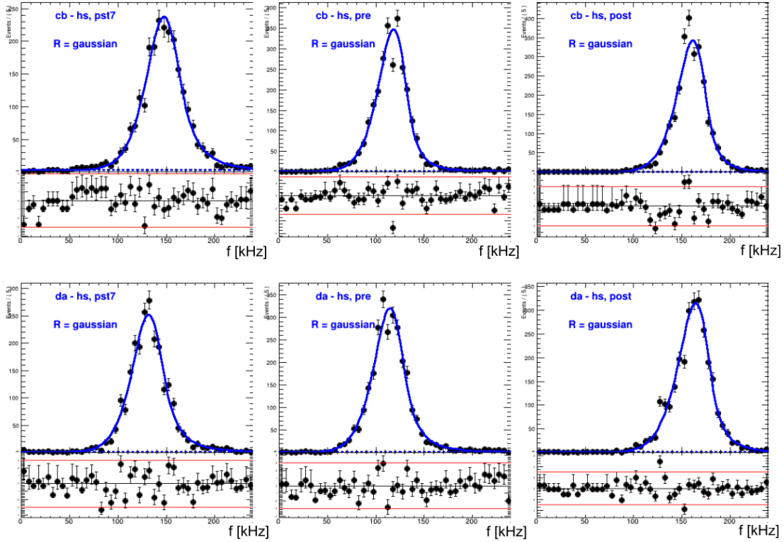
Figure 4.6: Fit results on the high statistics samples, with the shared k parameter left free to vary in the fit, and with shared \Delta f , to help the convergence of the fit.
