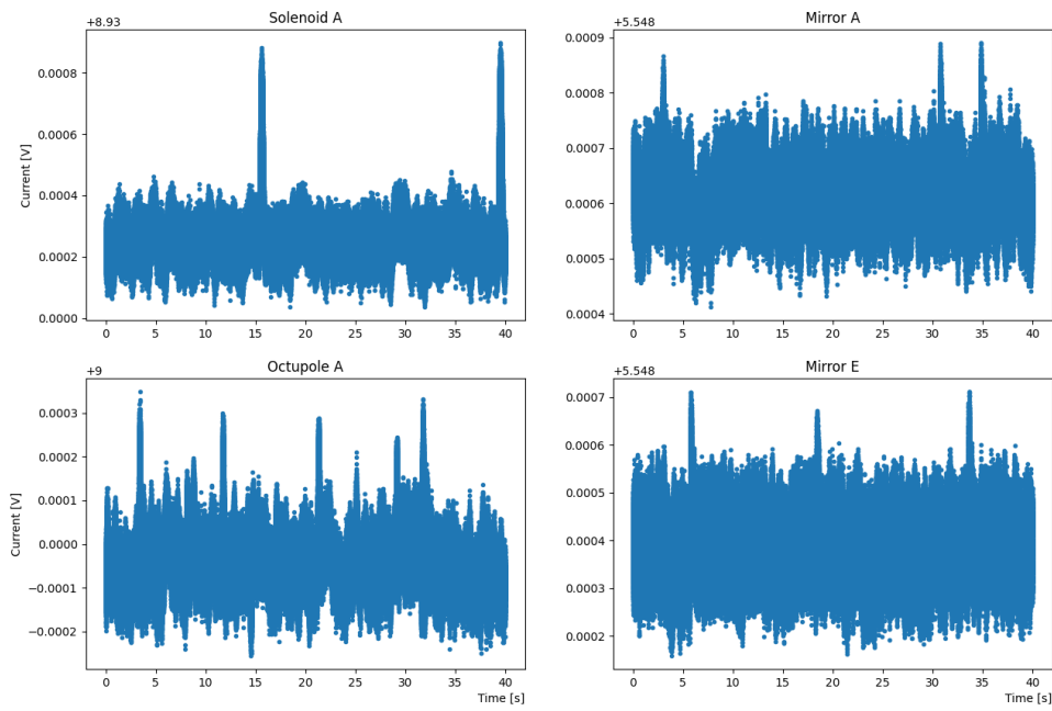
Figure 4.9: Example of DCCTs traces for a total of 40 second of acquisition. The units on the y-axis are Volts, since the DCCT provides a \pm 10 V output. The traces have been converted in Ampere units and the amplitude of the glitches has been used to study possible discrepancies on the measurement induced by change in the magnetic field minimum
