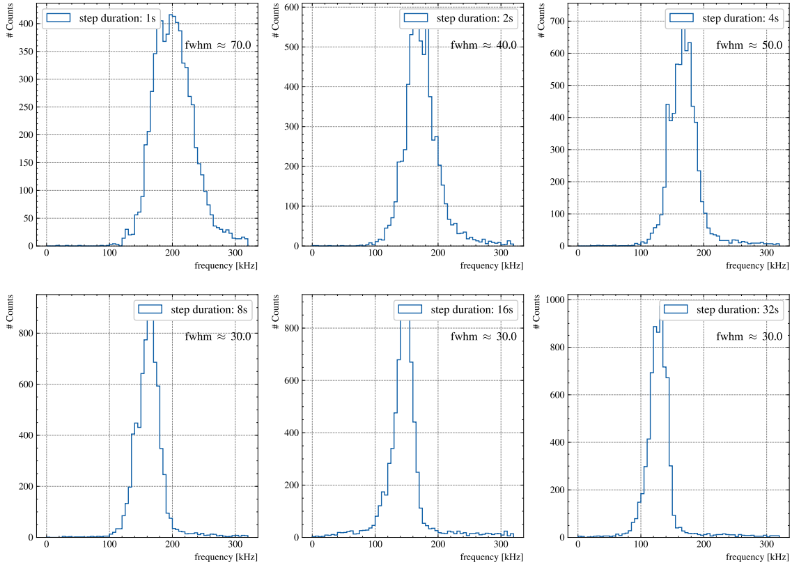
Figure 3.6: Collection of high statistic f_{cb} lineshapes measured for various pulse length duration. The starting frequency is expressed arbitrary to 0 kHz
