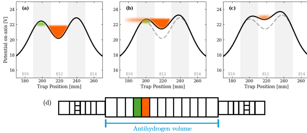
Figure 2.5: This picture illustrate the slow merge technique used to synthesize antihydrogen. Positron (orange cloud) and antiproton plasma (green cloud) are firstly in separated location as shown in (a). By slowly raising the central potential minimum, antiproton and positrons clouds meets, and antihydrogen is synthesized through 3 body recombination (b). The mixing phase ends with final potential state shown in (c), with some positrons still trapped, and used as diagnostic purpose (i.e to measure the final positron temperature after mixing). The duration of the mixing phase is typically in the range of few seconds, and it's a parameters tuned to maximize antihydrogen production. The shown figure is reproduced from [22]
