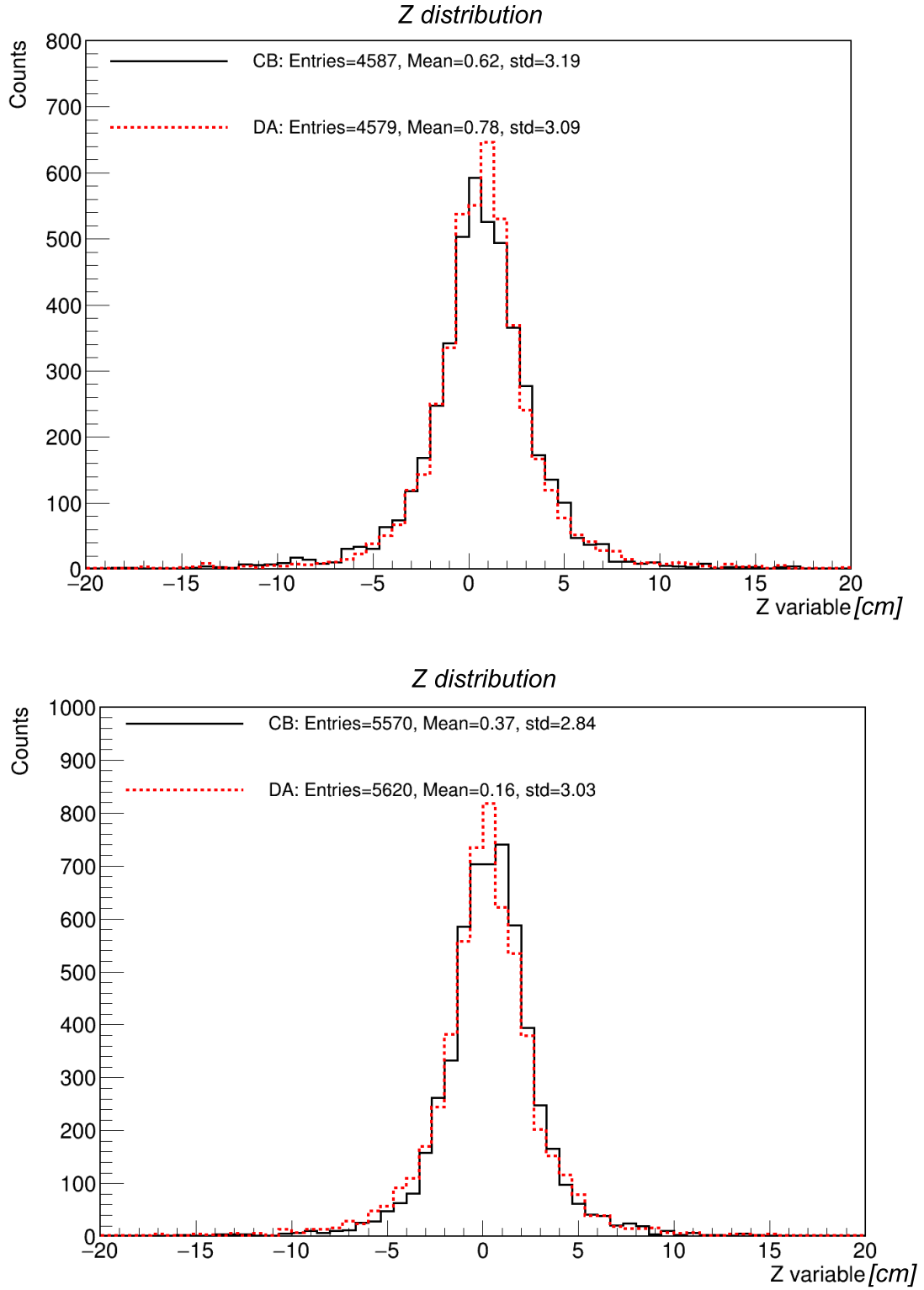
Figure 4.14: Distribution of Z variable of the annihilation vertices for the high field series (top) plot, and low field series (bottom plot). Each plot show two distribution: the Z distribution for annihilation during |c\rangle \rightarrow |b\rangle measurement (black continuous line) and during |d\rangle \rightarrow |a\rangle measurement (red dotted lines). The distribution contains all the accumulated events of the eight repetitions.
