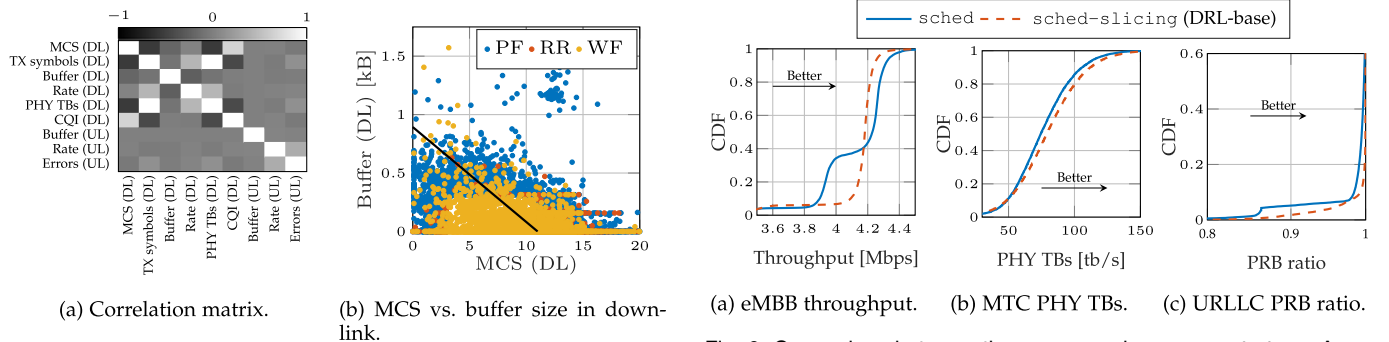
Fig. 5. Correlation analysis for the URLLC slice with 11 PRBs and the slice-based traffic profile. The solid line is the linear regression fit of the data.
