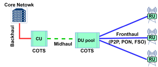
Fig. 5. O-RAN architecture.
