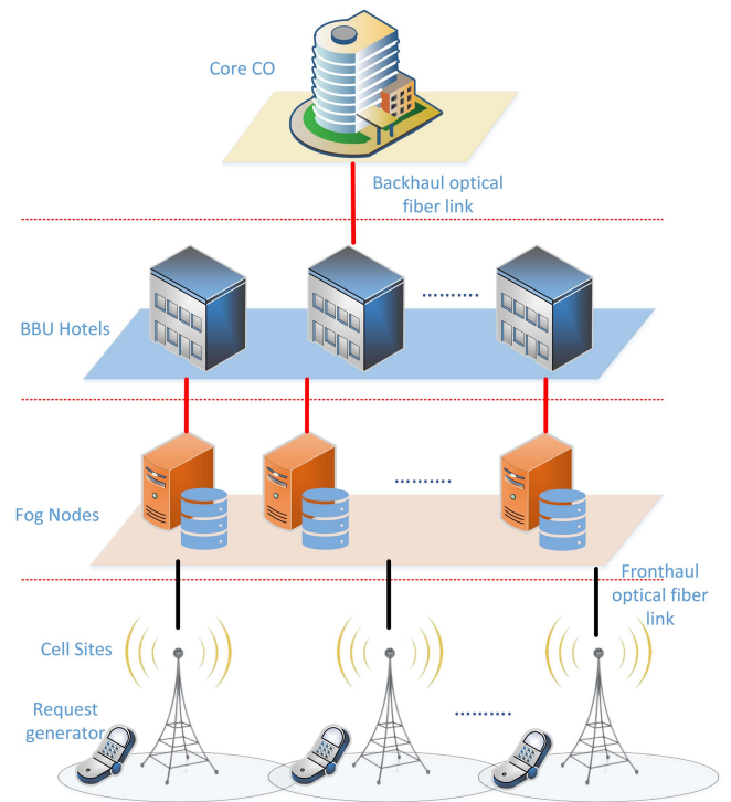
Fig. 1. Proposed cloud fog RAN (CF-RAN) over WDM architecture.
