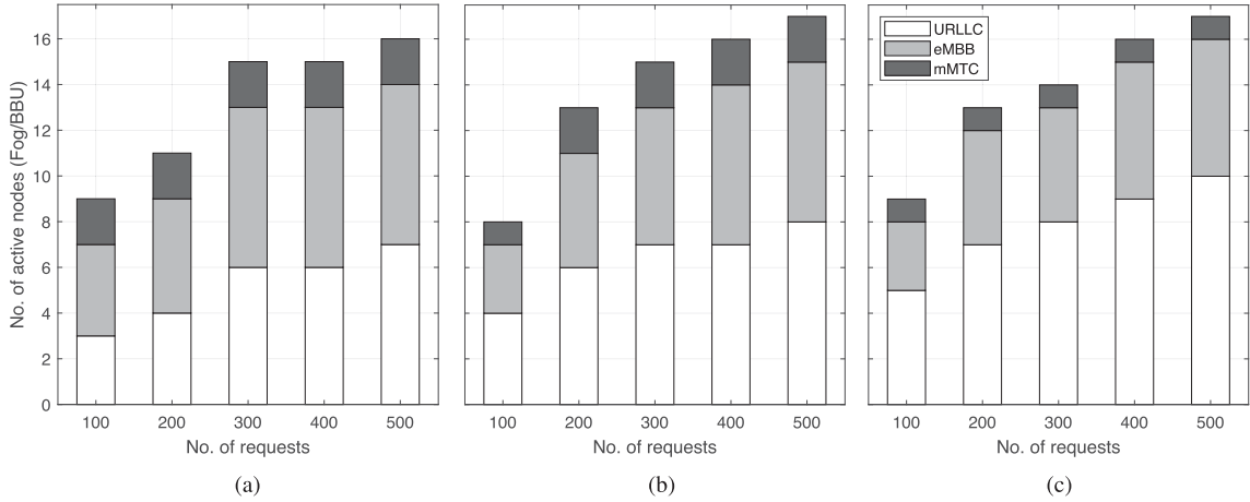
Fig. 12. Number of active nodes w.r.t. total number of requests for ILP in 3-layer architecture for different \alpha values. (a) \alpha = 0.25 . (b) \alpha = 0.5 . (c) \alpha = 0.75 .
