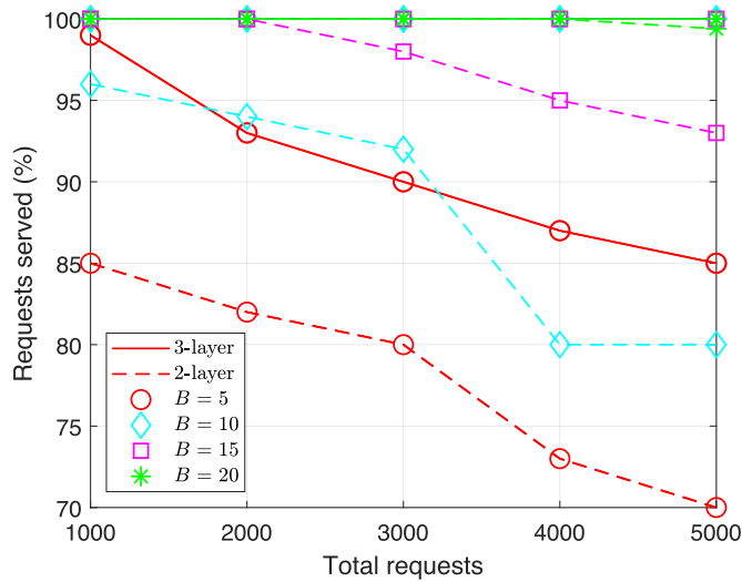
Fig. 10. Comparison of 3- and 2-layer approaches in terms of served requests vs. the total number of requests.
