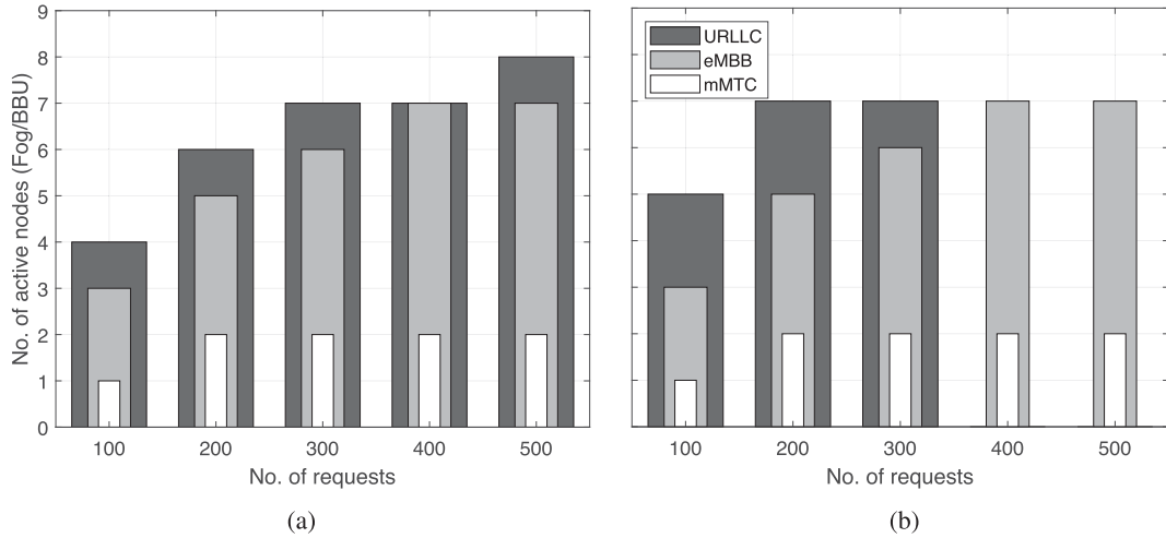
Fig. 4. Number of active nodes for ILP. (a) 3-layer architecture. (b) 2-layer architecture.
