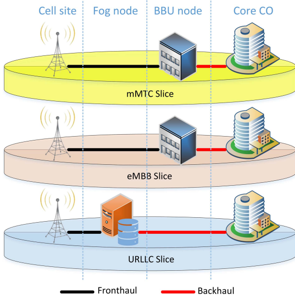
Fig. 3. Network slicing considering three traffic types.
