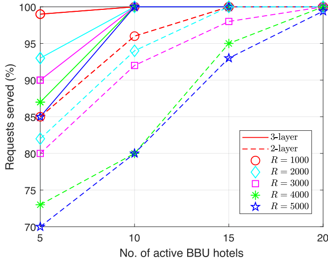
Fig. 9. Comparison of 3- and 2-layer approaches in terms of served requests vs. the total number of BBU hotels.
