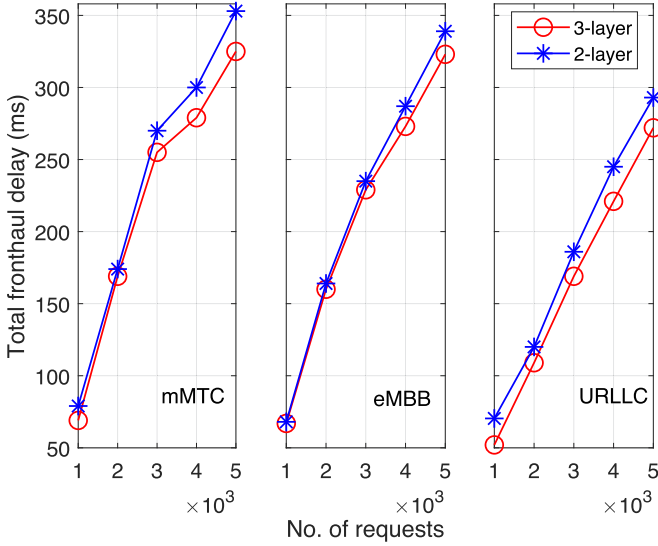
Fig. 6. Comparison between 2-layer and 3-layer architecture in terms of total fronthaul delay for heuristic algorithm.
