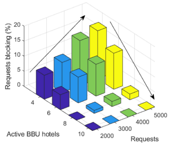
Fig. 8. Request blockage rate for 3-layer approach.
