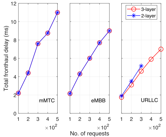
Fig. 5. Comparison between 2-layer and 3-Layer in terms of total fronthaul delay for ILP.
