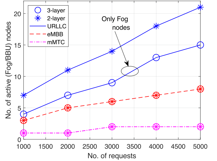
Fig. 7. Comparison between 2-layer and 3-layer architecture in terms of number of active nodes for heuristic algorithm.
