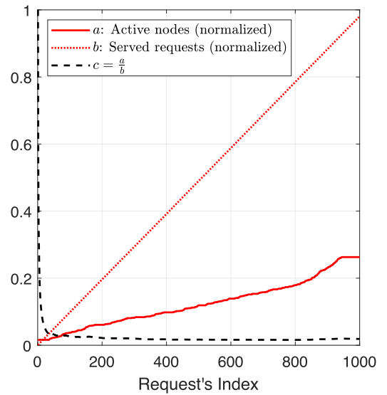
Fig. 13. Convergence of Algorithm 1.
