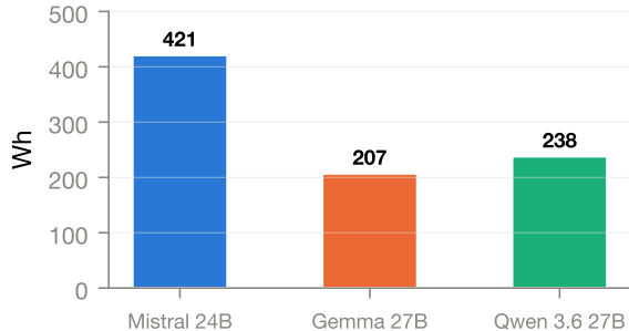
Energy per Resolved Instance
