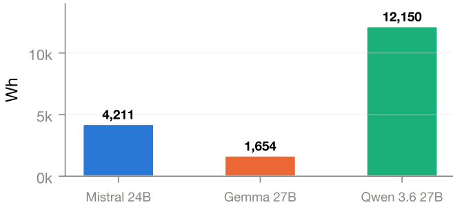
Total GPU Energy
