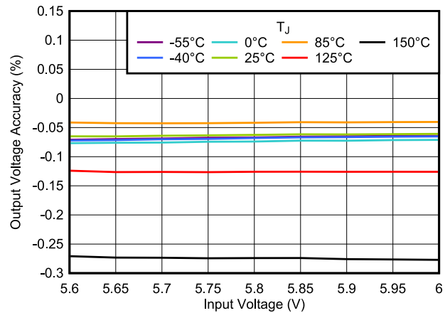
Figure 5-22. Output Voltage Accuracy vs V_{IN}
