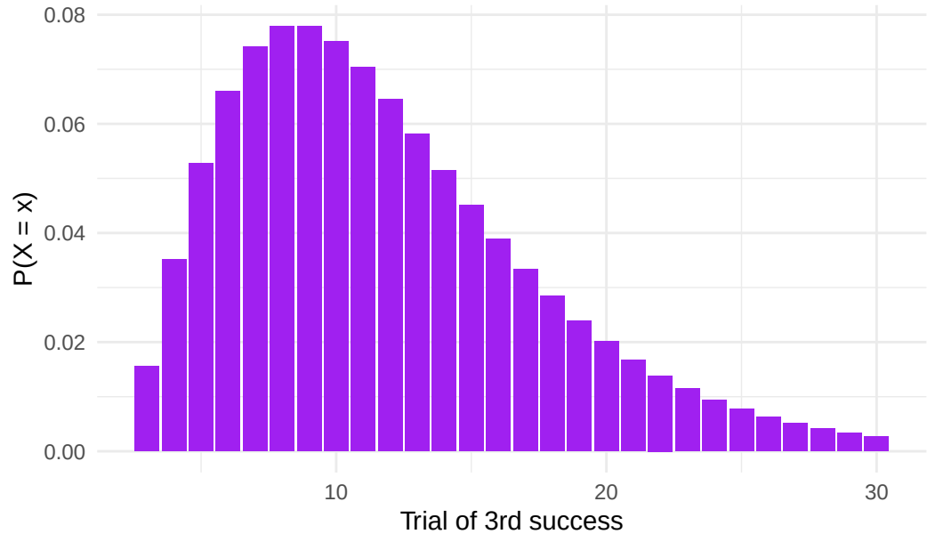
Negative Binomial( r = 3 , p = 0.25 )
