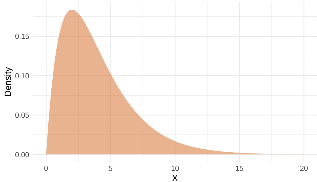
Chi-square(df = 4)
