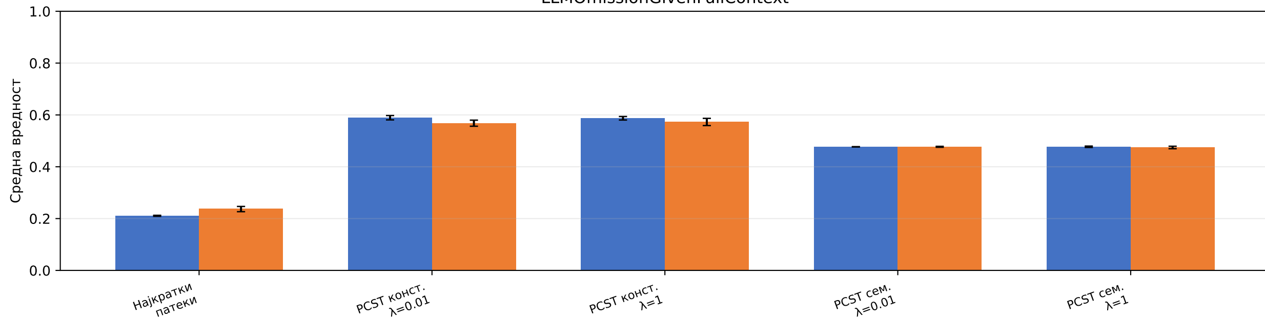
LLMOmissionGivenFullContext
