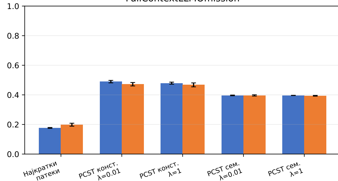
FullContextLLMOmission
