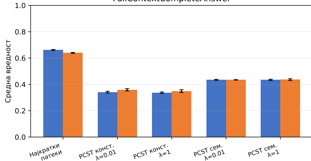
FullContextCompleteAnswer
