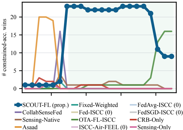
(a) round-mean CRB
