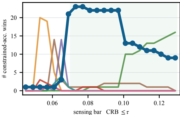
(b) final-round CRB
