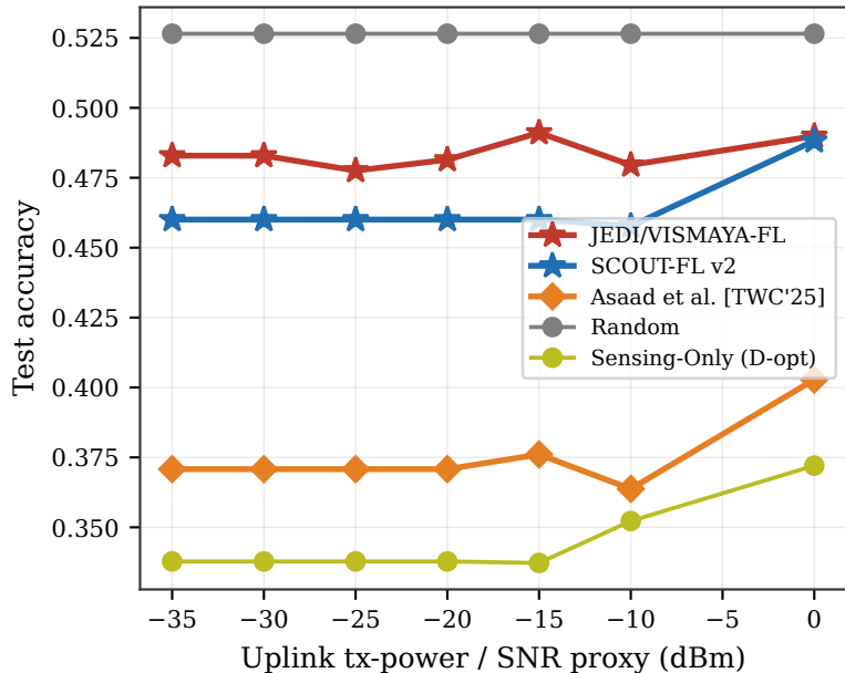
(a) Accuracy vs link quality
