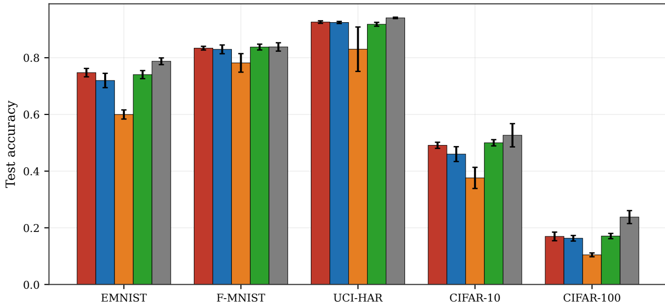
Accuracy across datasets (K/N=10%, 150 rd, 5 seeds)
