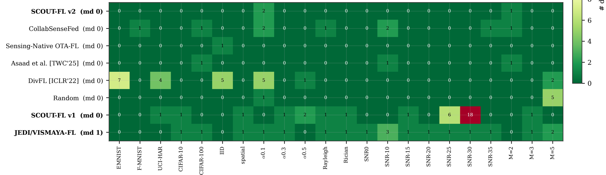
# strict dominators (final-round CRB); 0 = Pareto-optimal
