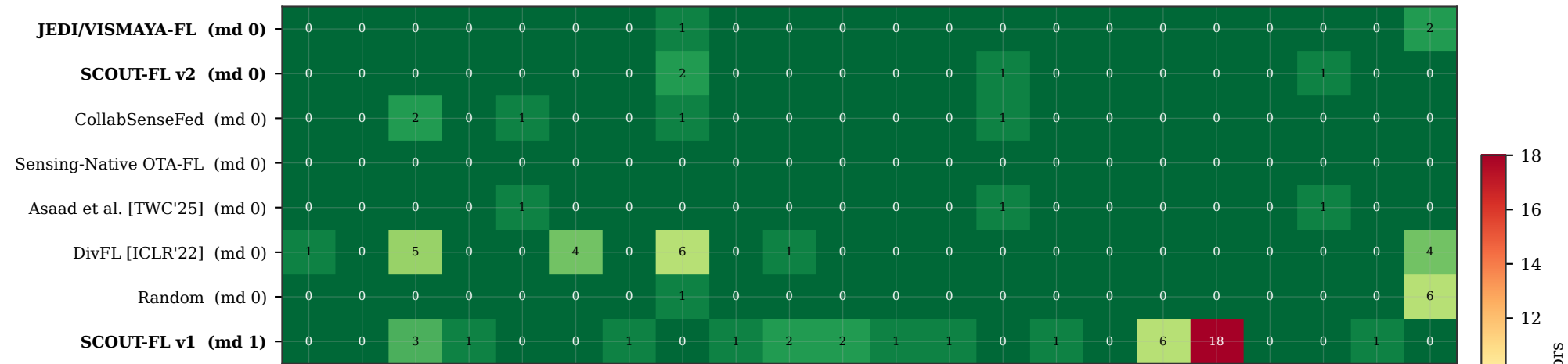
# strict dominators (round-mean CRB); 0 = Pareto-optimal
