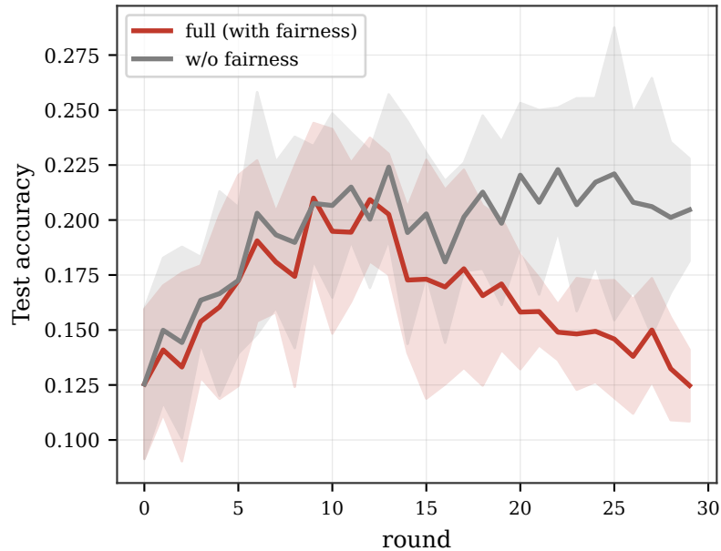
(a) Accuracy (mean \pm 95% CI)
