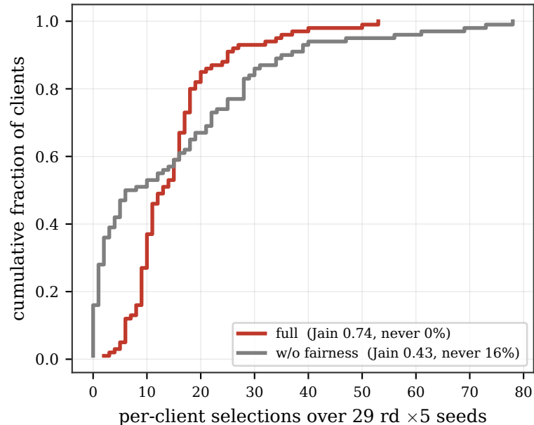
(c) Participation CDF (K=100); flatter-left = more starvation
